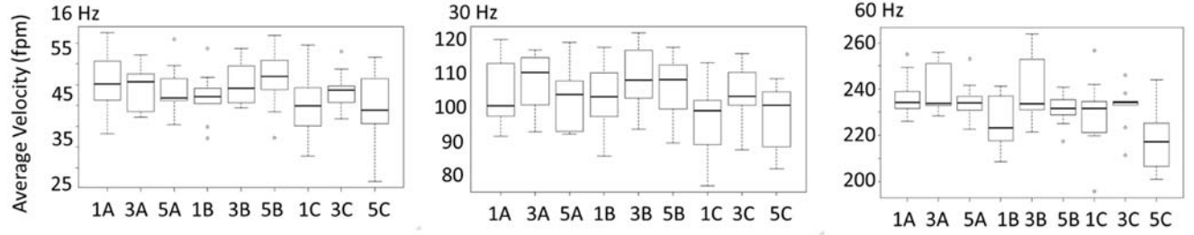
Figure 13. Variance of Velocity Profiles for with Flow Straighter Data
