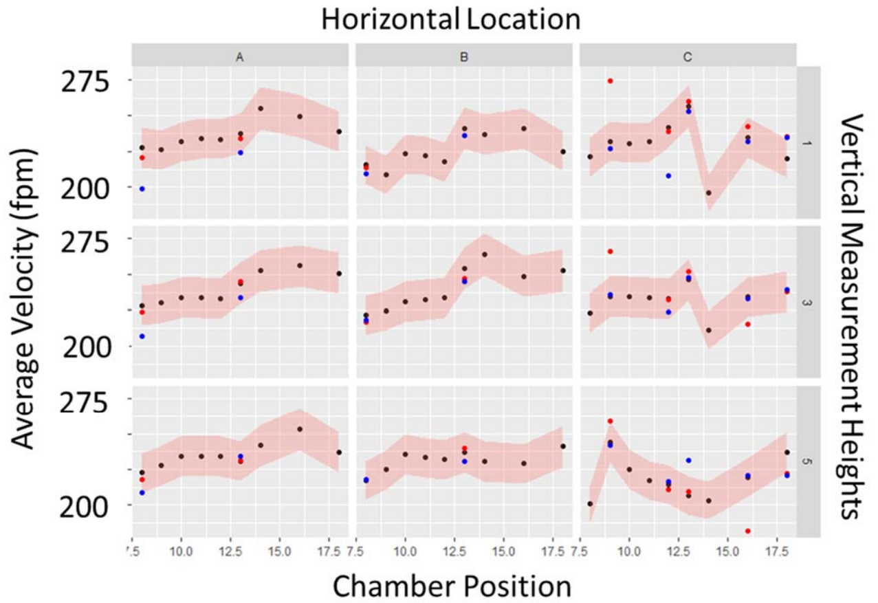
Figure F4. Day-to-Day Variability in Average Velocity at 60 Hz, with Flow Straightener
