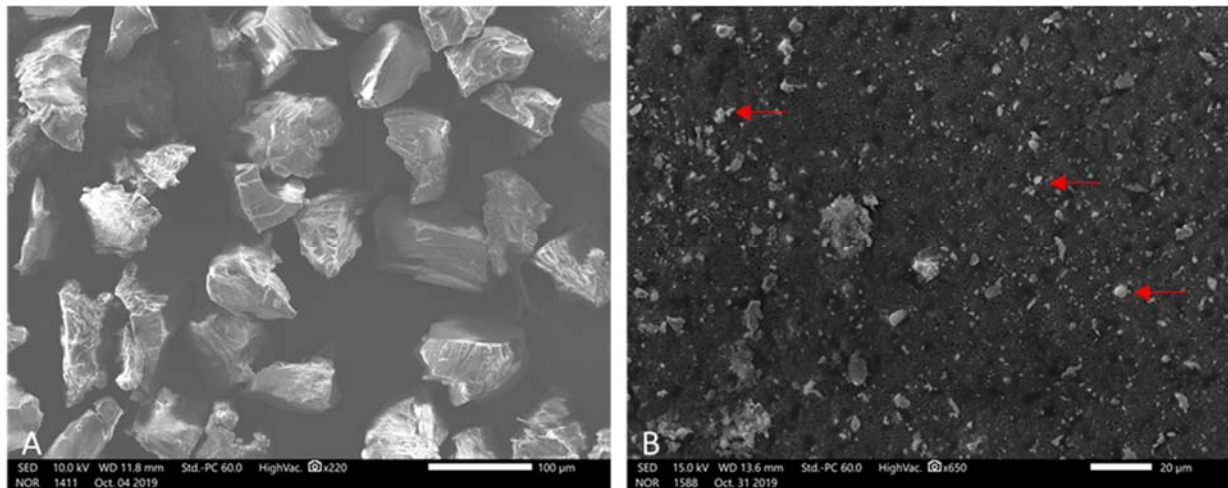
Figure 17. Micrographs: A) Bulk Dust; B) IOM Filter F, Red Arrows Showing Bright Particles
